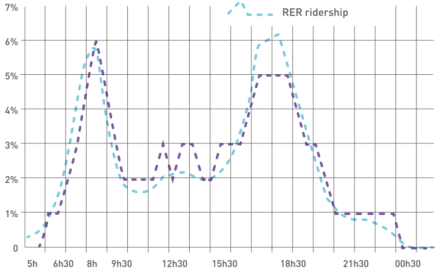
Figure 9 : Hourly traffic distribution in Metro and RER systems in Ile-de-France Region 7
