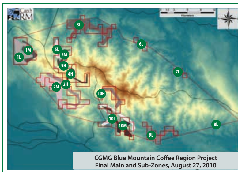
Figure 2.4. Homogeneous risk zones (16 sub-zones) in the Blue Mountain pilot area
